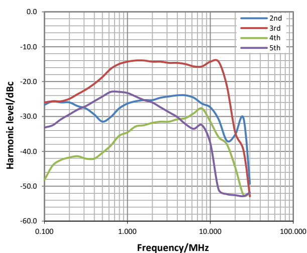
Harmonics
