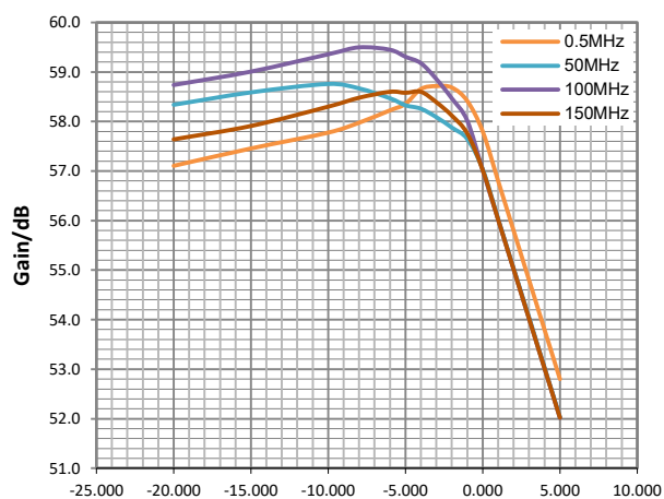
Gain as a function of input power
